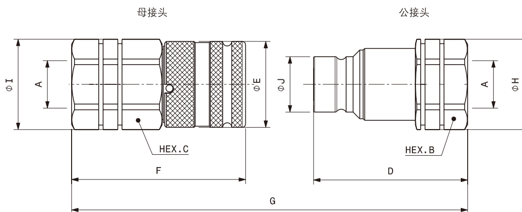
螺纹接口：内螺纹SAE (ISO 11926-1 &amp; SAE J1926-1)
