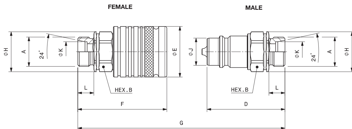
Port description: MALE THREAD METRIC L SERIES – 24° CONE (ISO 8434-1 & DIN 2353)
